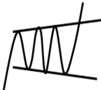
broadening formation
